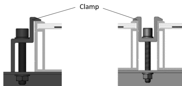
End clamp installation
